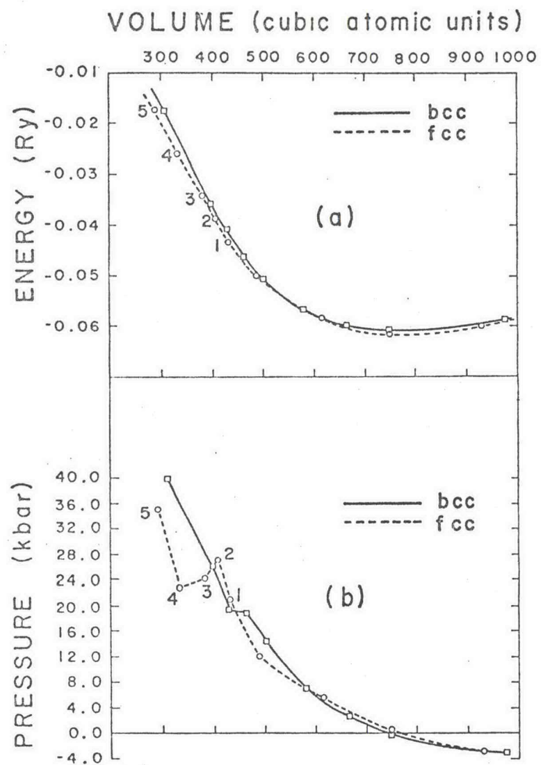
FIG. 1. Cs cohesive energy and pressure.
