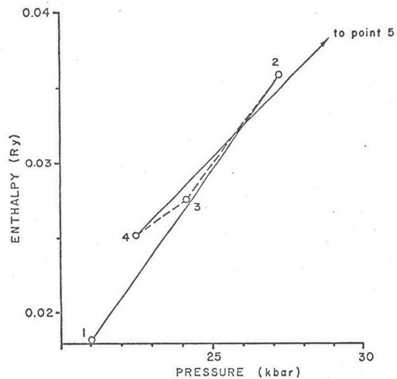
FIG. 2. Cs enthalpy.
